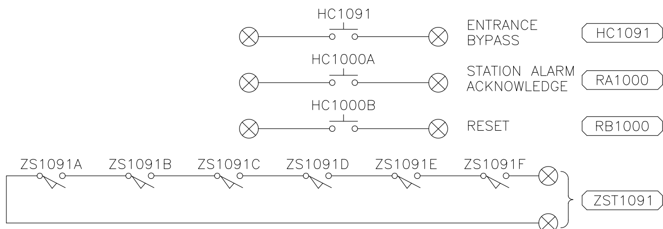
CP-10 ELEMENTARY DIAGRAM (A) E10.6
